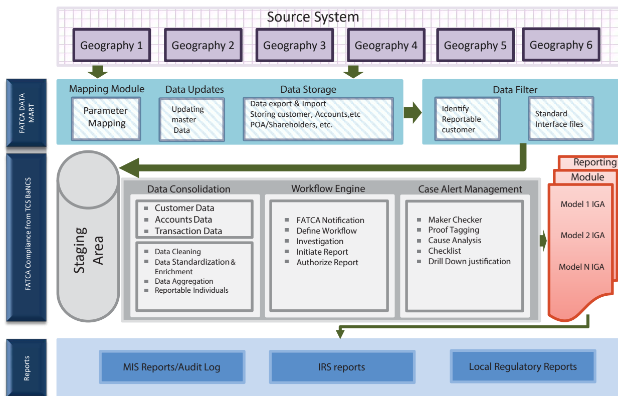
Figure 1: An overview of the FATCA Compliance solution
